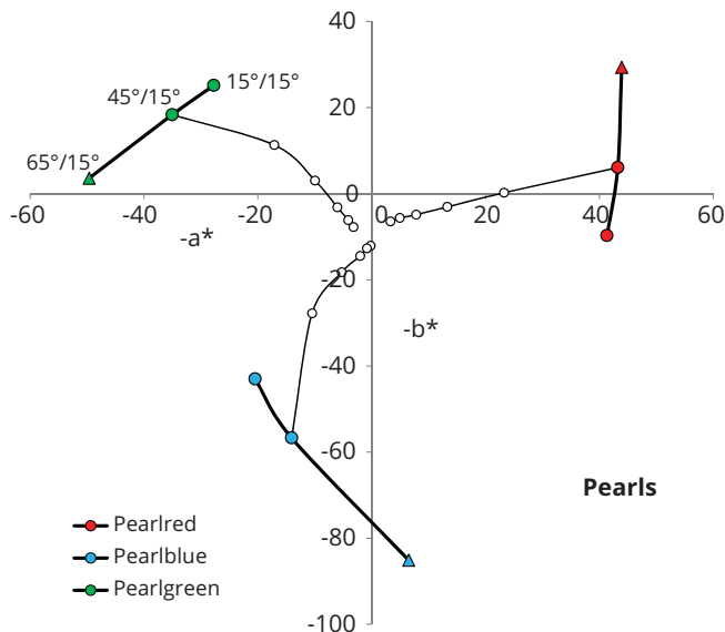
FIGURE 6 » The shift to shorter wavelengths is also evident in the representation of the a^*b^* values. For colored interference pigments, the color shifts counterclockwise when the illumination is flatter with the same angular difference to the gloss – for example, the pearlgreen from yellow-green to blue-green, the pearlred from blue-red to yellow-red.
