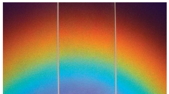
FIGURE 8 » Typical image of a polychromatic rainbow, which starts as blue-violet at an illumination angle of 35° or above.
